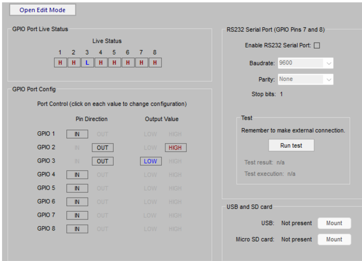
Figure 51: I/O Ports
