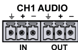
Figure 8: CH1 Audio
