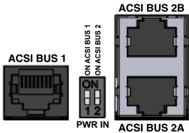
Figure 9: ACSI Bus
