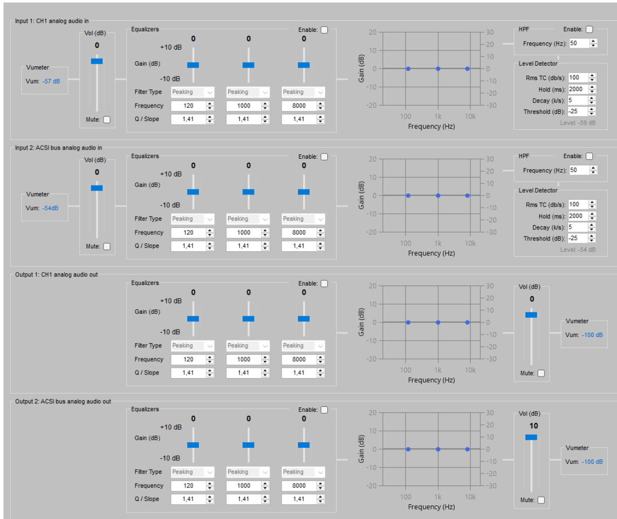
Figure 39: DSP Config
