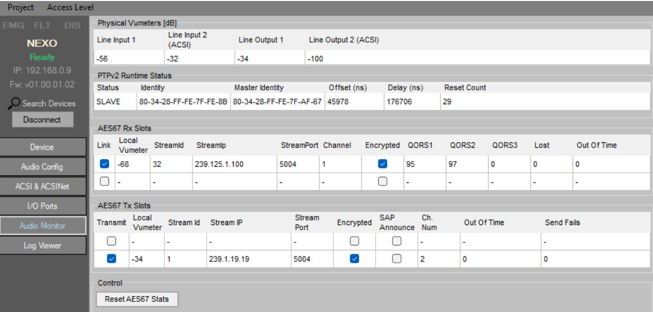
Figure52: Audio Monitor
