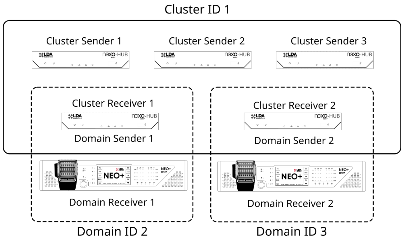
Figure 24: ACSiNet System
