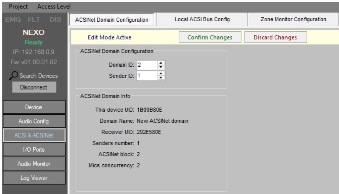
Figure 41: ACSINet domain
