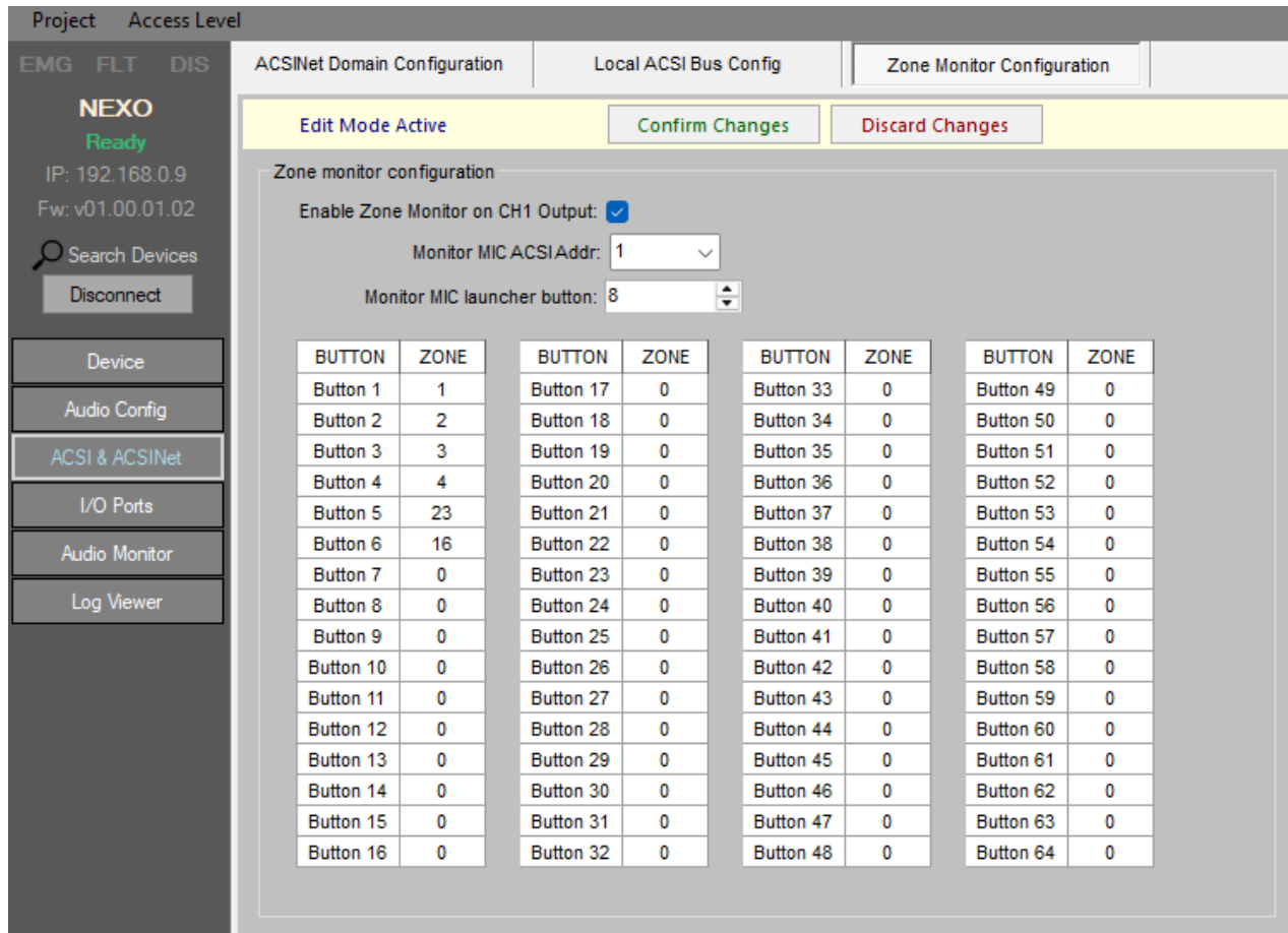
Figure 50: Zone Monitor
