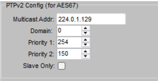
Figure 53: PTPv2 Config
