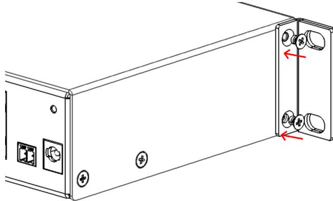
Figure 16: Short fixing bracket assembly
